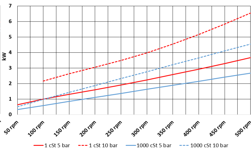
Absorbed power
