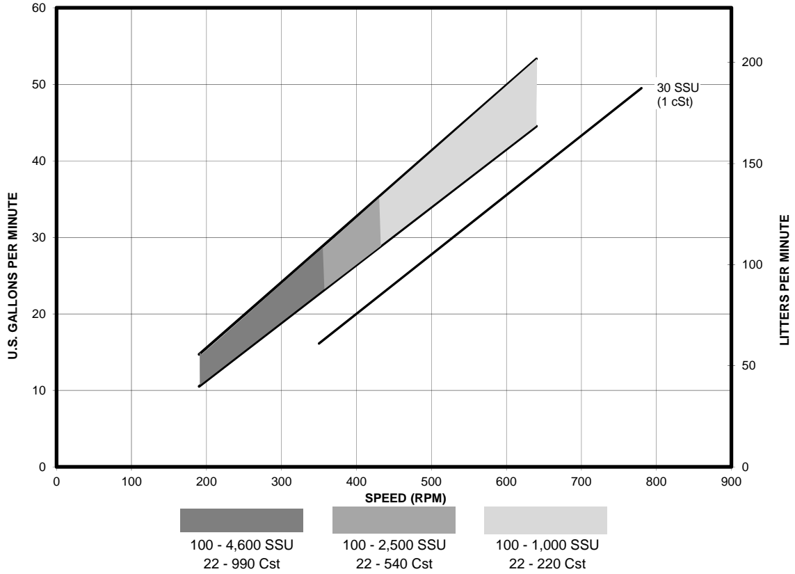
FLOW AT 50 PSI (3.45 Bar)
