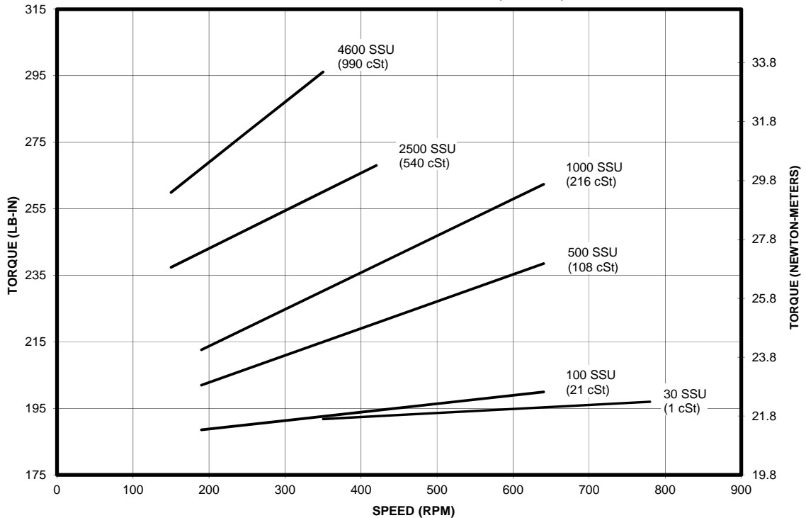
TORQUE REQUIRED AT 50 PSI (3.45 Bar)
